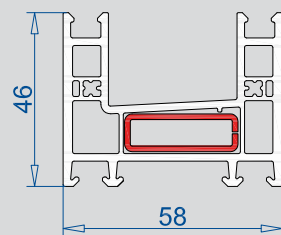
Marco 105.370 Ref. 113.020
