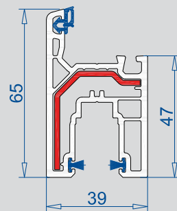
Hoja 105.373 Ref. 113.074
